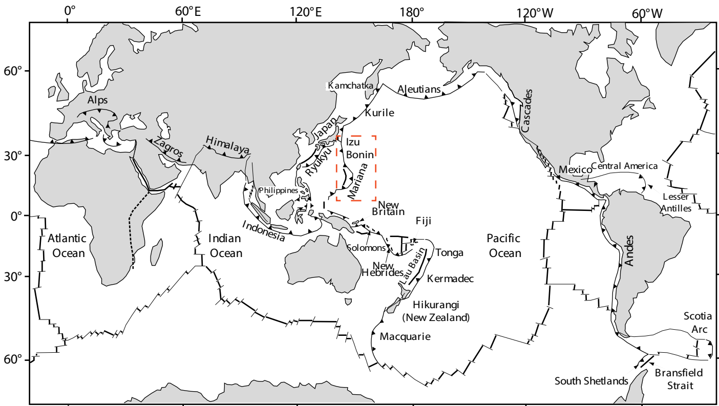
Fig. 1: Convergent margins of the world. Barbed lines mark convergent plate margins, teeth are on the overriding plate. Continental collision zones (marked with *) are a kind of convergent plate margin although these are not considered here. Spreading ridge (divergent plate margins) abbreviations: JdFR: Juan da Fuca ridge; EPR: East Pacific Rise; PAR: Pacific-Antarctic Ridge; SEIR: SE Indian Ridge; SWIR: SW Indian Ridge; CR: Carlsberg Ridge. Dashed box shows location of Izu-Bonin-Mariana convergent margin.
